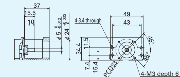
Fig 27 Mounting dimension for motor attachment of TU...E (Low profile type)
