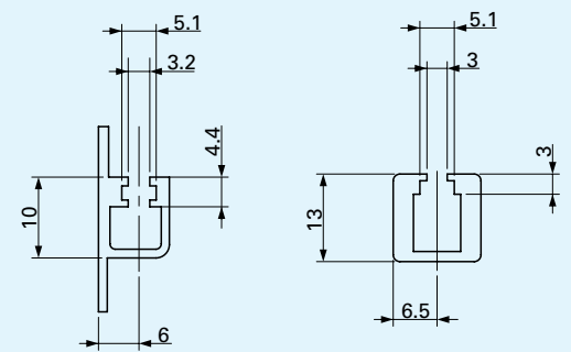
Fig. 4 Sectional shape of sensor rail
