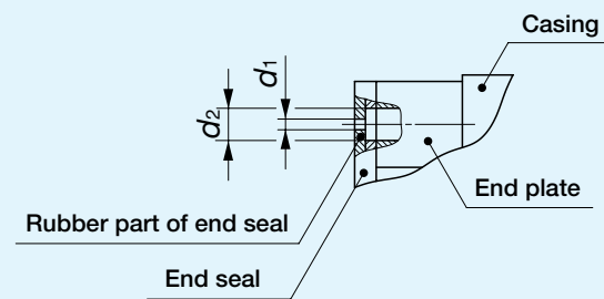
Fig. 8 Oil hole
